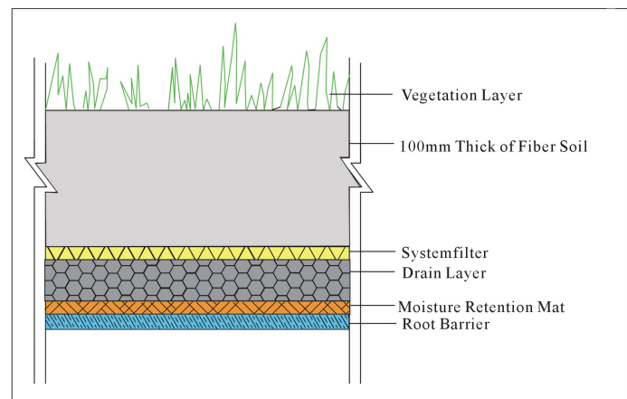
Green Roof System Section Drawing
