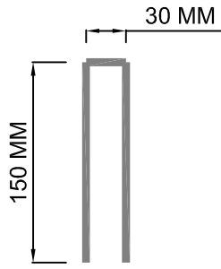
DETAIL OF U-SHAPE STAPLE
