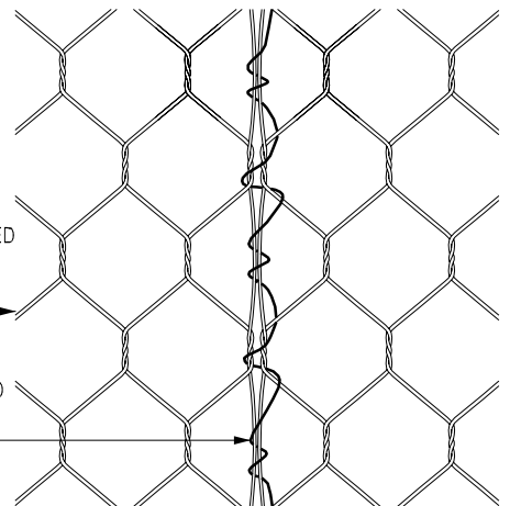
LACING OF ADJACENT MESH SHEETS
