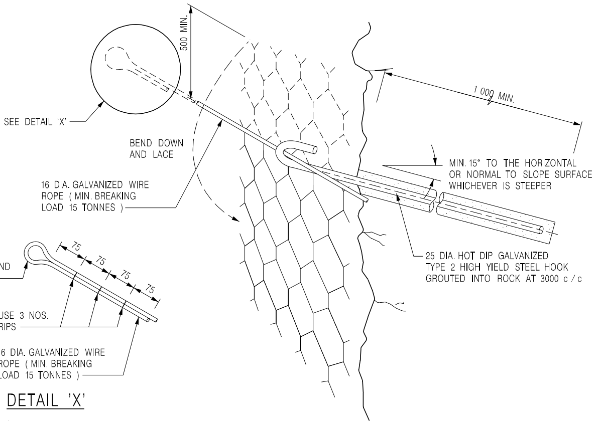
FIXING AT TOP
