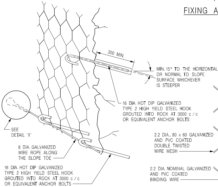
FIXING MESH TO FACE AND AT BOTTOM OF FACE
