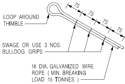
DETAIL 'X'
