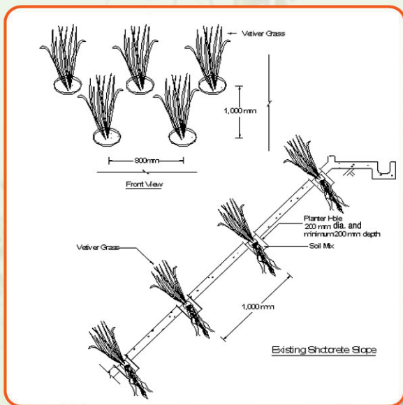
Application on shotcrete slope
