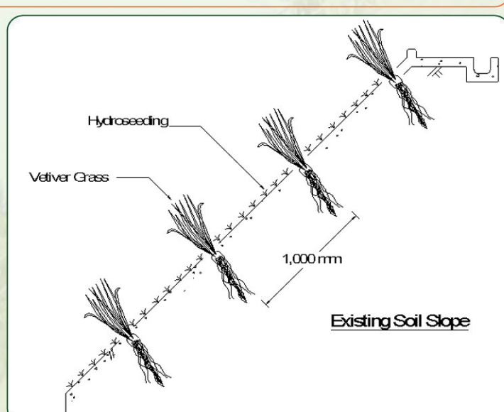
Application on soil slope for erosion control
